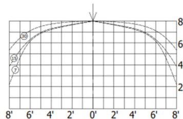
1/2" Orifice - K=5.6
